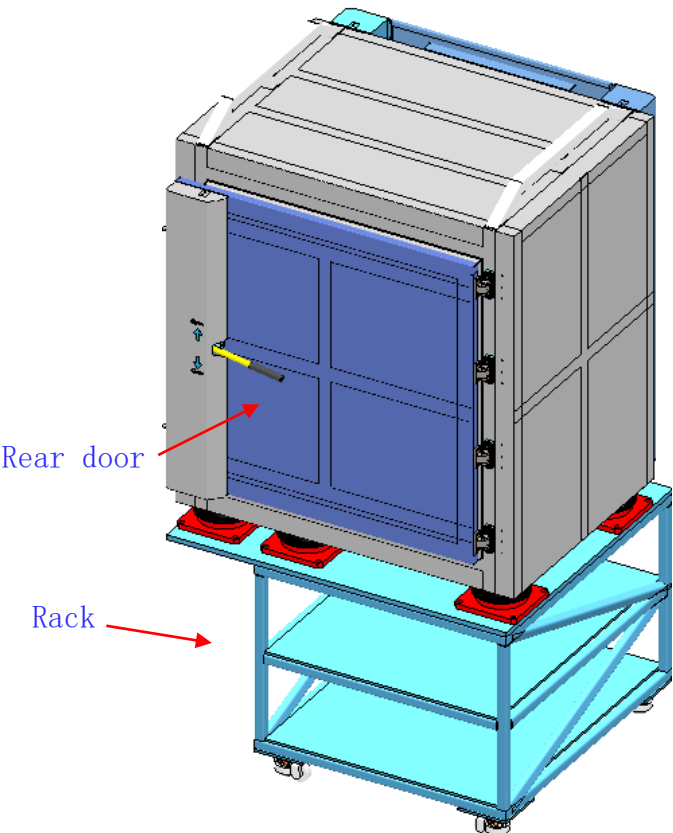
Rear view
